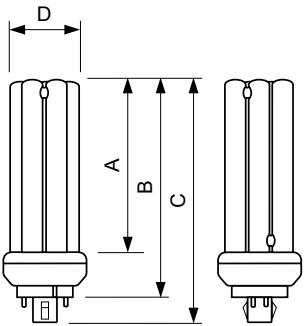
PL-T ALTO 26W/841/4P A
