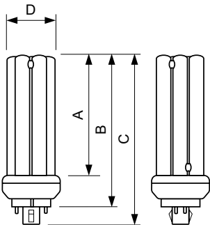
PL-T ALTO 57W/841/4P A
