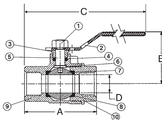
T-585-70-CP NPT x NPT
