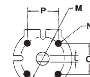
TOP FLANGE FOR 1/2" THRU 2"
