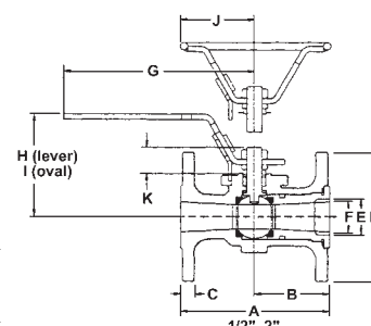
F-530-S6-R-66-FS Stainless x Stainless Flanged
