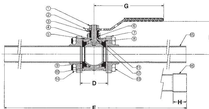
CS-595-YX/CS-595-YX-EC CSE x CSE
