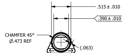
DETAIL A TOP INK MARKING INK COLOR: PINK PER SPEC #: F921
