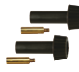
70161 2 Replacement Knobs Black Finish With 1/2" Extensions Tapped 3/16"-F x 3/16"-M
